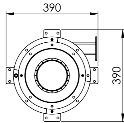
VIEW J
