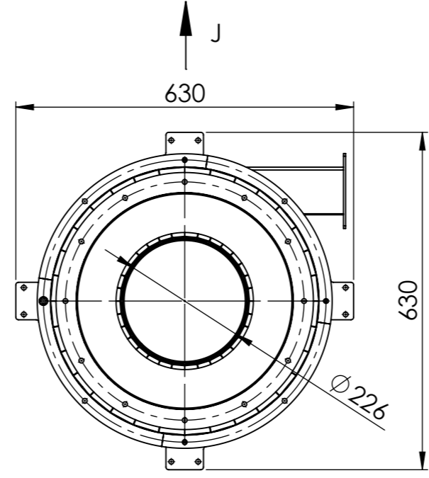
VIEW J
