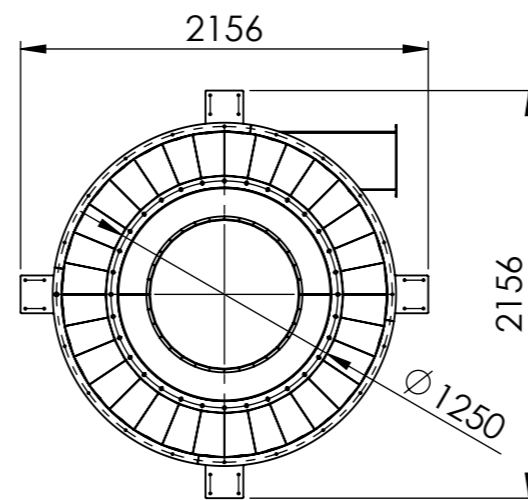
VIEW J
