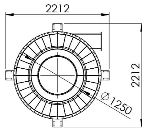
VIEW J
