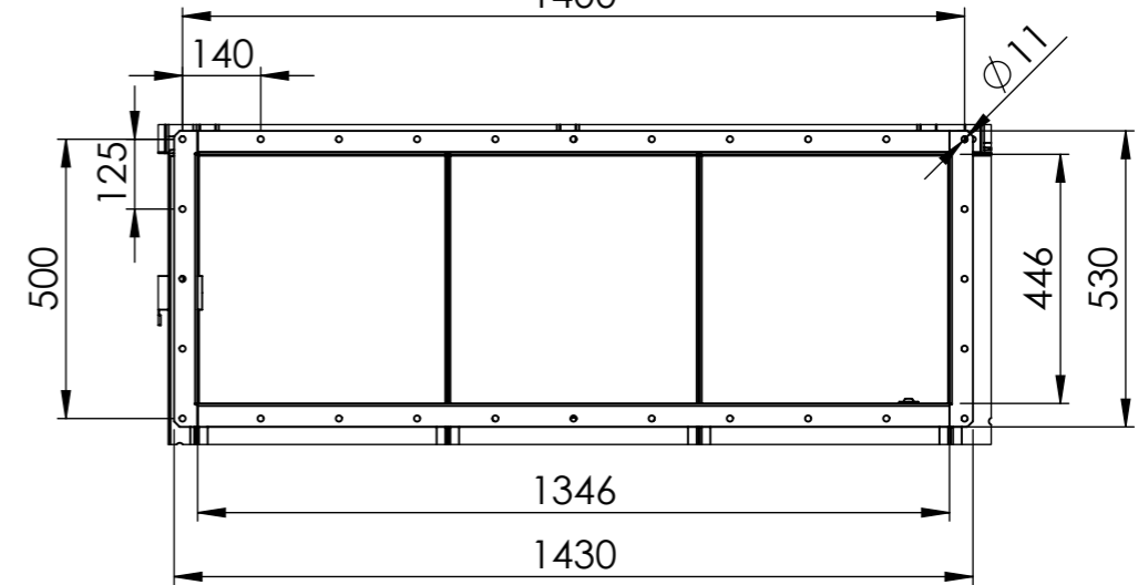
DETAIL B OUTPUT FLANGE 1400
