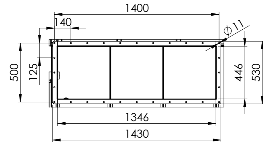
DETAIL B OUTPUT FLANGE
