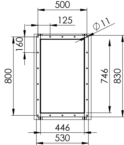
DETAIL A 2x INPUT FLANGE
