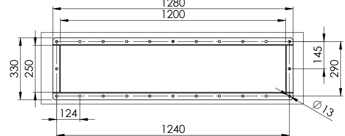
DETAIL B INPUT FLANGE
