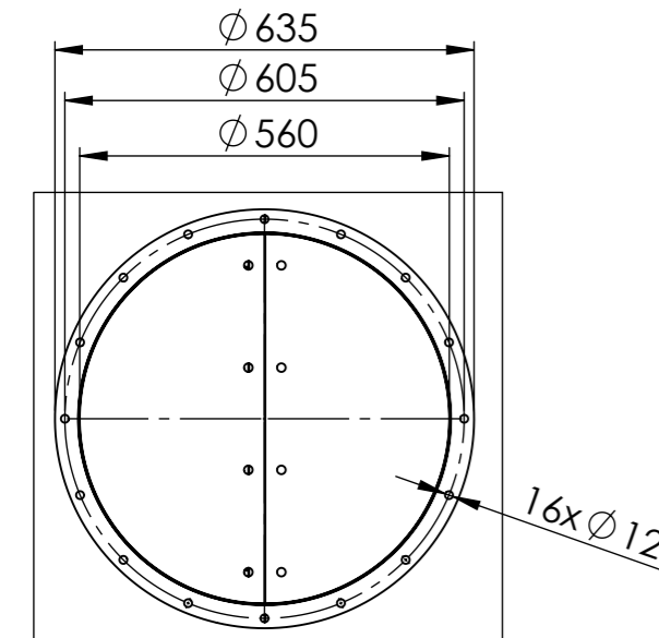
DETAIL A OUTPUT FLANGE
